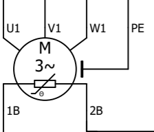
Gearmotor + thermistor
