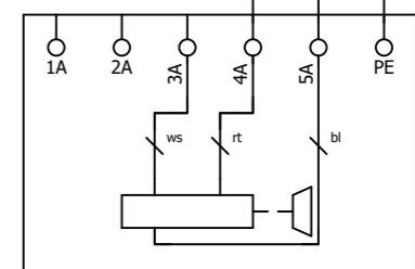
Brake 24VDC
